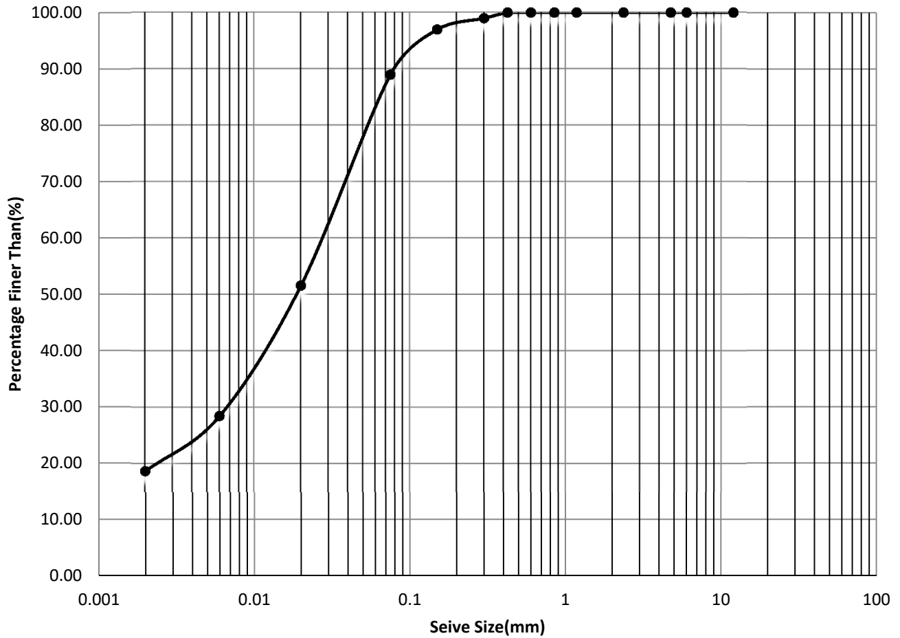
GRAIN SIZE CURVE
